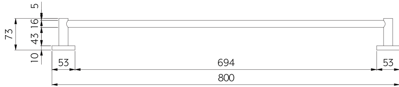
SIDE VIEW
